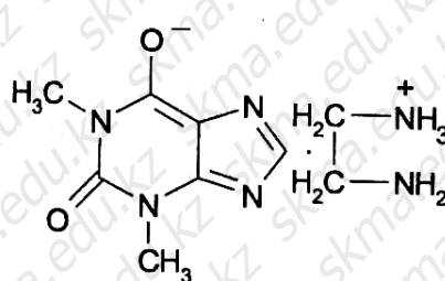
Euphillinum
