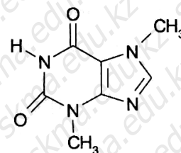
Theobrominum
