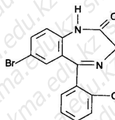
Phenazepamum
